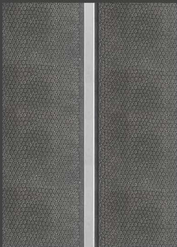
Mercury
