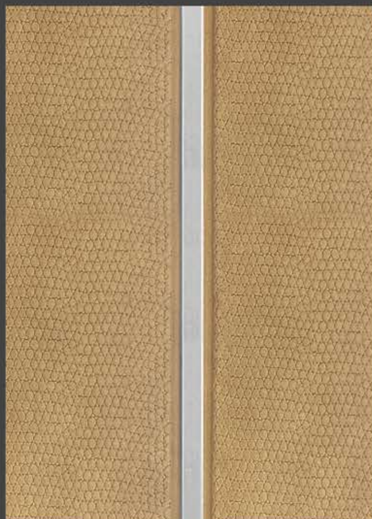
Saturn
